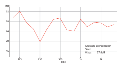
隔聲測試 Sound insulation test
