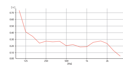
混響測試 Reverberation time test
