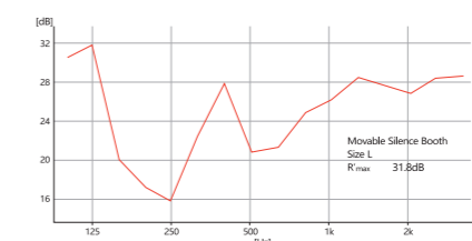
隔聲測試 Sound insulation test
