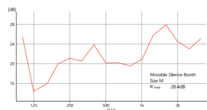
隔聲測試 Sound insulation test
