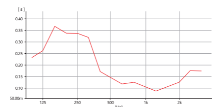
混響測試 Reverberation time test
