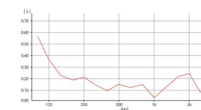
混響測試 Reverberation time test
