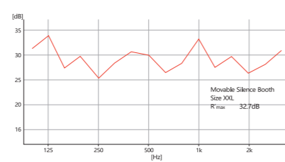
隔聲測試 Sound insulation test
